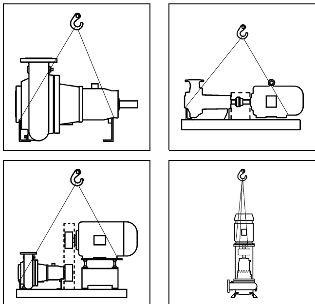
Proper handling
