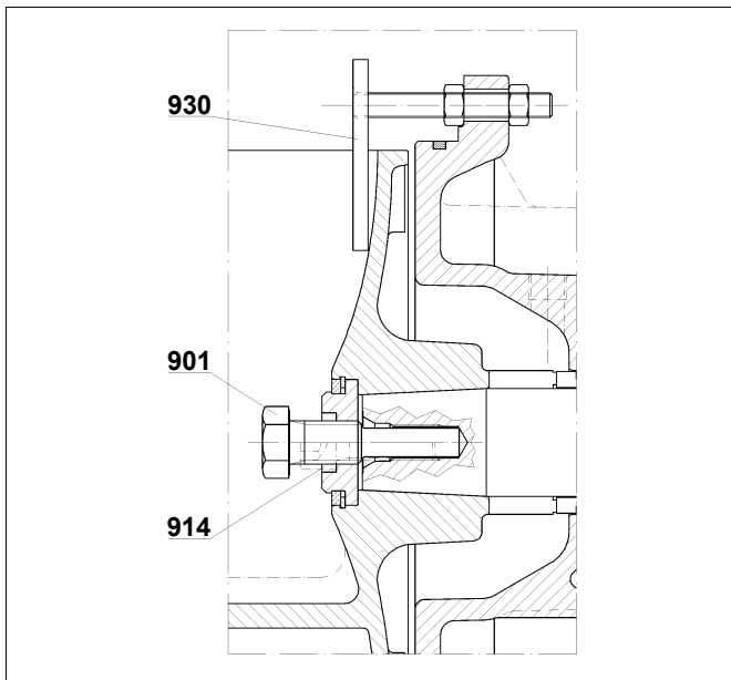
Sketch of impeller disassembly
